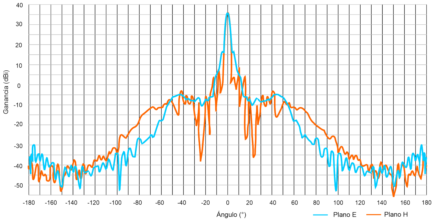
Antena NetPoint NP64 (NP6-SDP-4FT)
